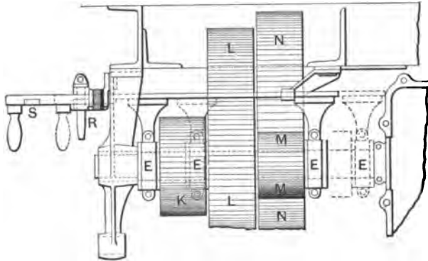
FIG. 274.—Change Speed Gear used on the Thornycroft Steam Wagon.
